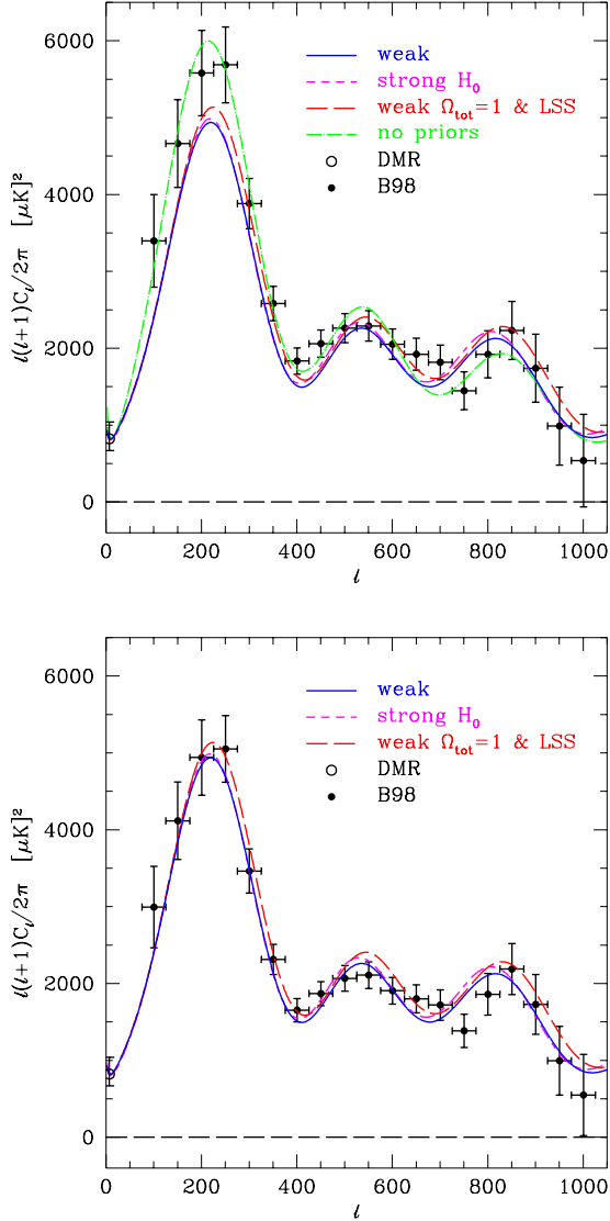
Fig. 3.— Selected best fit models normalized to the best compromise amplitude between COBE-DMR and BOOMERANG are shown overlayed on the BOOMERANG spectrum. The upper panel shows the points plotted as listed in table 3. The “no priors” best fit model ( \Omega_{tot} = 1.15, H_0 = 42, \Omega_\Lambda = 0.7, \omega_b h^2 = 0.020, \omega_c h^2 = 0.060, t_0 = 20 Gyr ) fits the central values very well with no calibration or beam shift, but has an unacceptably low value for H_0 . Once the weak priors are invoked, the remaining models take advantage of the uncertainty in calibration and beam size to maintain a good fit. The parameter estimation algorithm allows calibration shifts and marginalizes over them, weighted as a Gaussian error. To demonstrate the effect, in the lower panel the points have been replotted with a 12% change in calibration ( 0.6\sigma ) and a 0.5 arcminute change in beam size ( 0.4\sigma ). The plot makes it clear that the best-fit conventional CDM models are indeed good fits to the data, once beam and calibration uncertainties are correctly accounted for.
